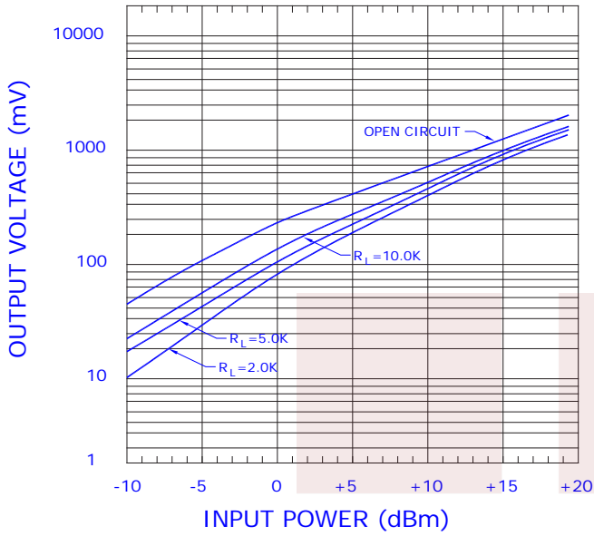
Transfer Curve
