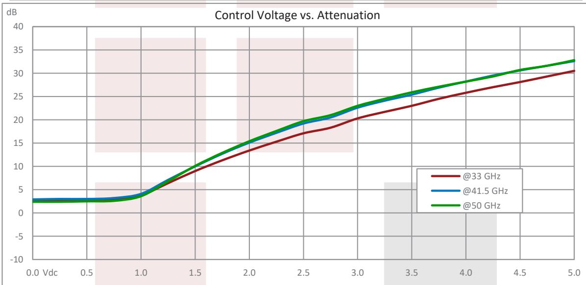
WR-22 Waveguide Voltage Variable Attenuator, Q Band, 33 GHz to 50 GHz, 0 to 30 dB Attenuation, 2.7 dB Loss, UG-383/U Flange
