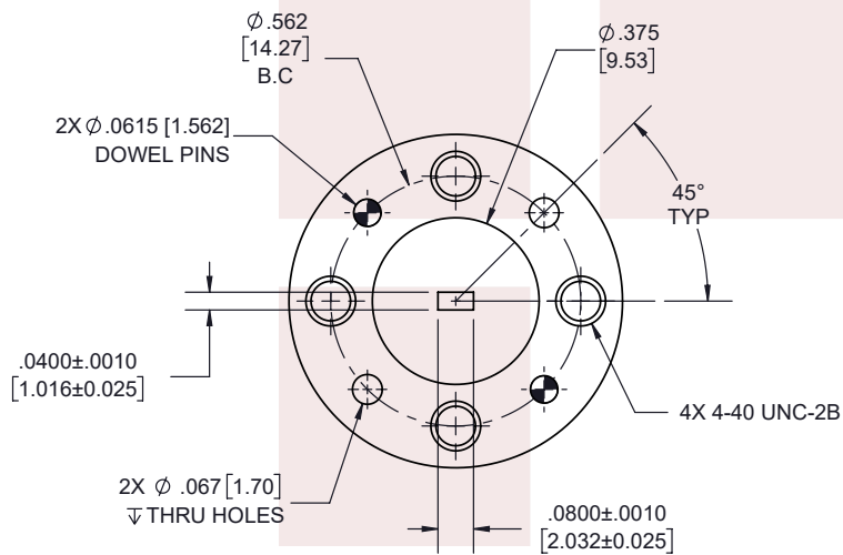
FLANGE DETAIL
