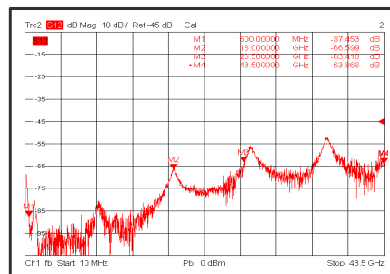
Isolation @-40°C
