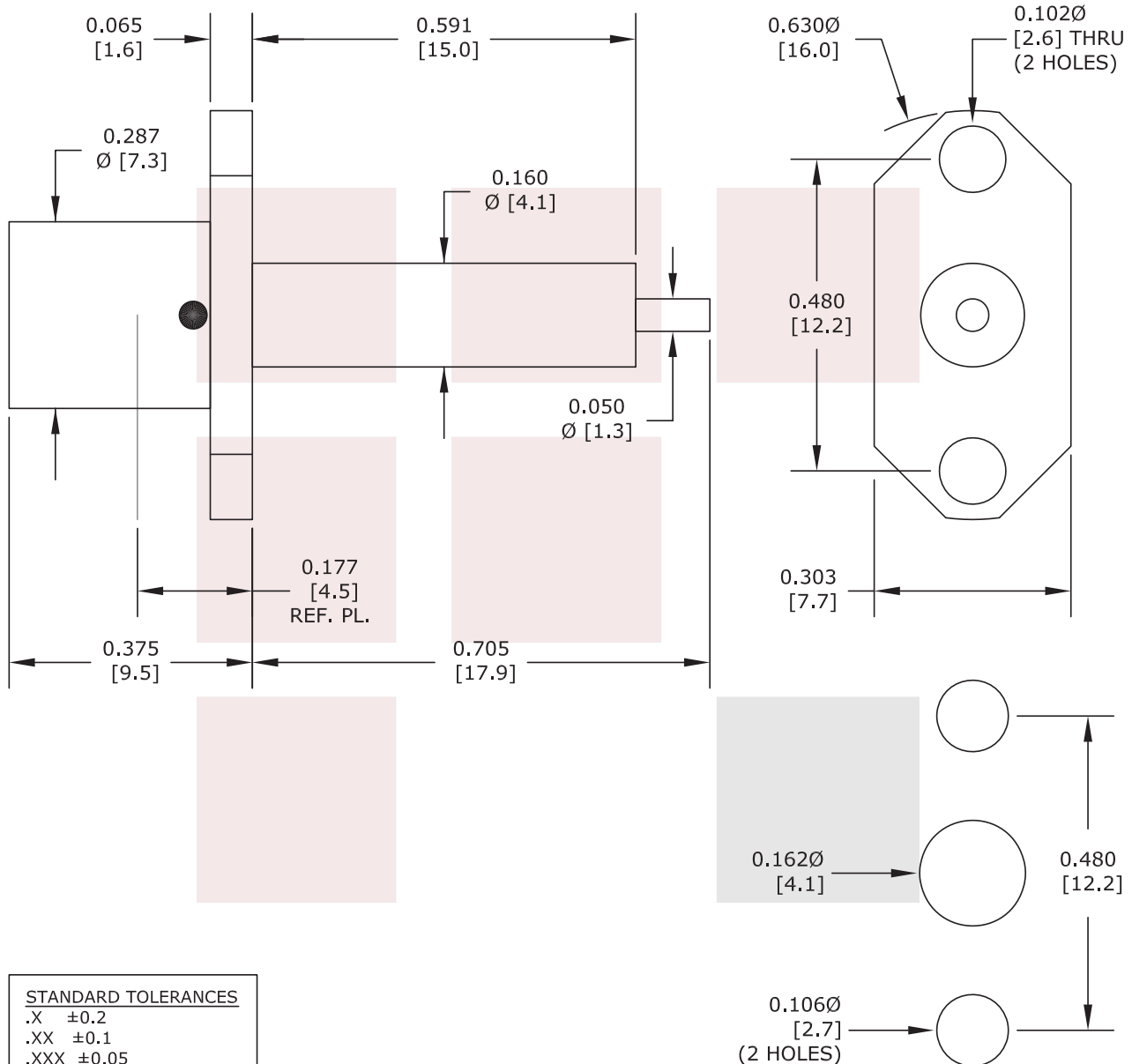
MOUNTING HOLES
