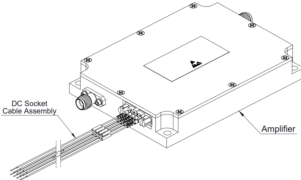
illustration of Amplifier & DC Socket Cable Assembly. Cable Assembly model FM15J000 sold separately (Picture shown for Reference Only)
