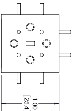
PORT 4 "DIFFERENCE"
