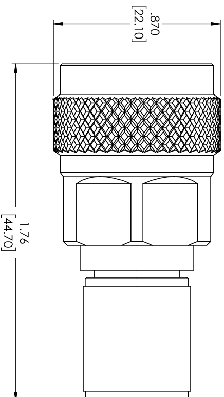
TYPE N MALE TERMINATION
