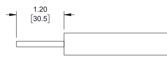
STRIPPING DIMENSIONS
