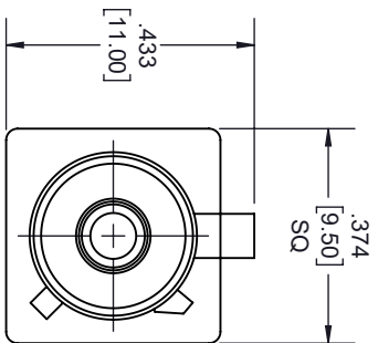
FAKRA PLUG H CODING VIOLET
