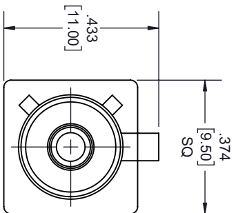
FAKRA PLUG D CODING BORDEAUX
