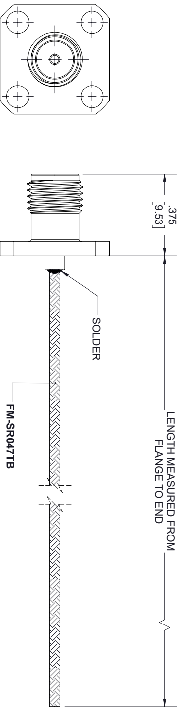
SMA FEMALE 4 HOLE FLANGE
