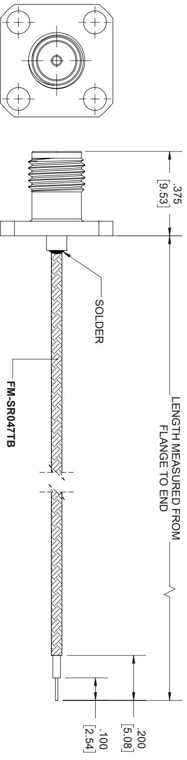
SMA FEMALE 4 HOLE FLANGE
