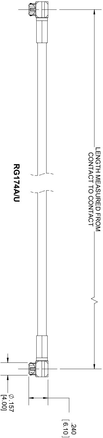
MMBX PLUG RIGHT ANGLE
