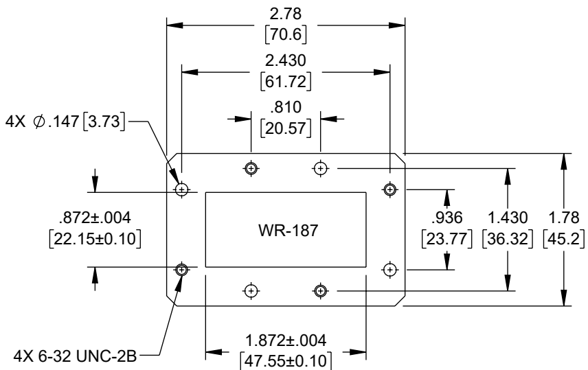
FLANGE DETAIL
