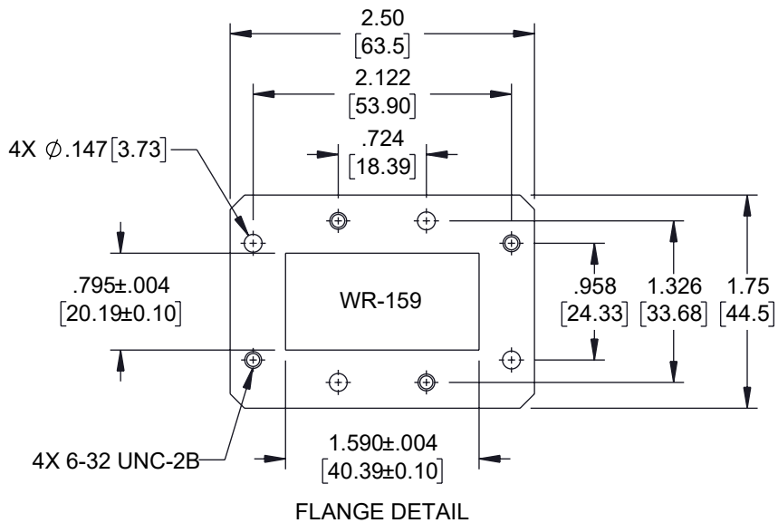
FLANGE DETAIL
