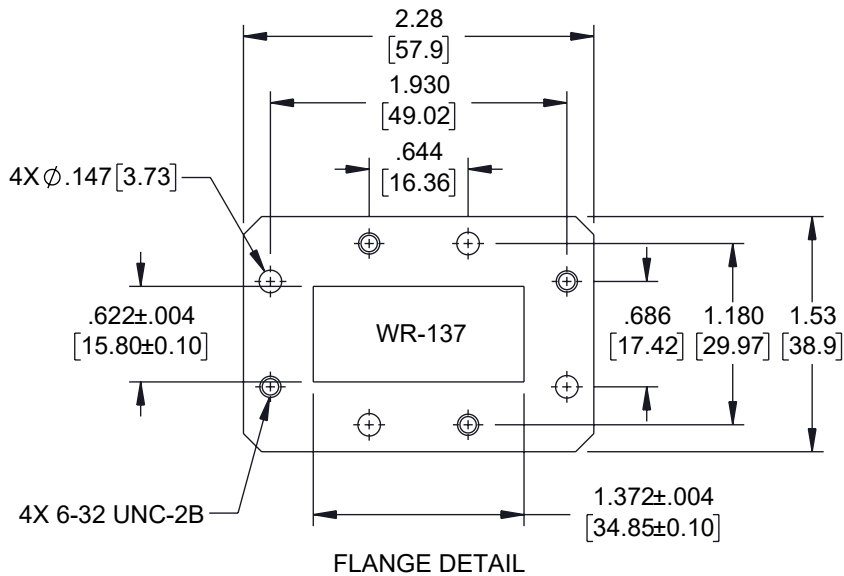
FLANGE DETAIL
